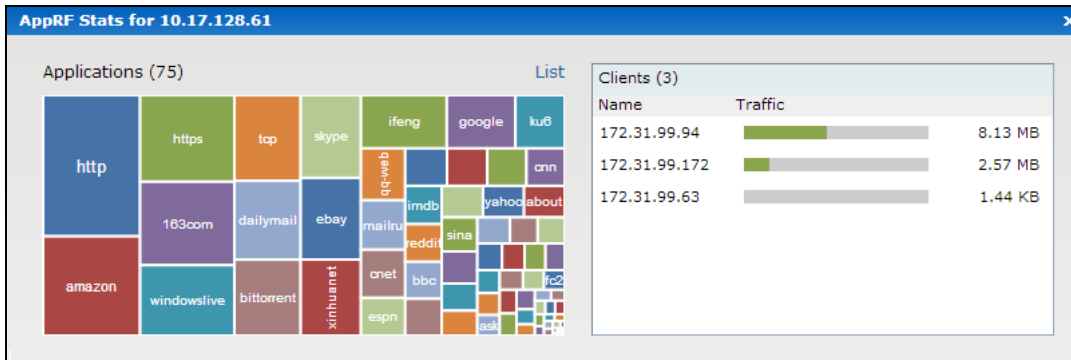
Figure 64 Application Chart - AP View
